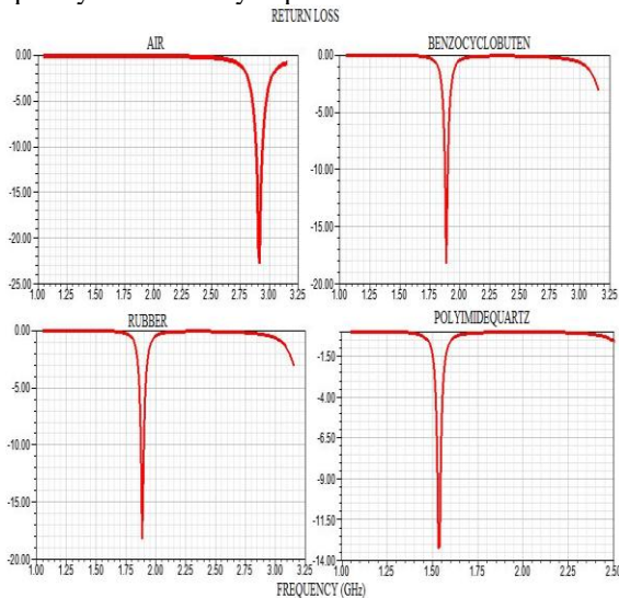
Fig 3: Return loss
