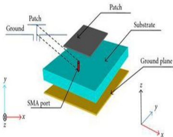
Fig 1: Coaxial Feed
