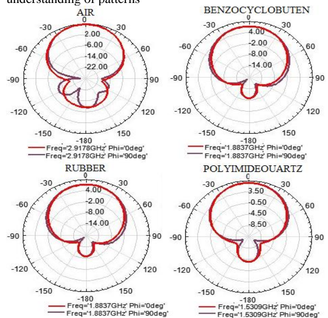
Fig 5: Radiation pattern
